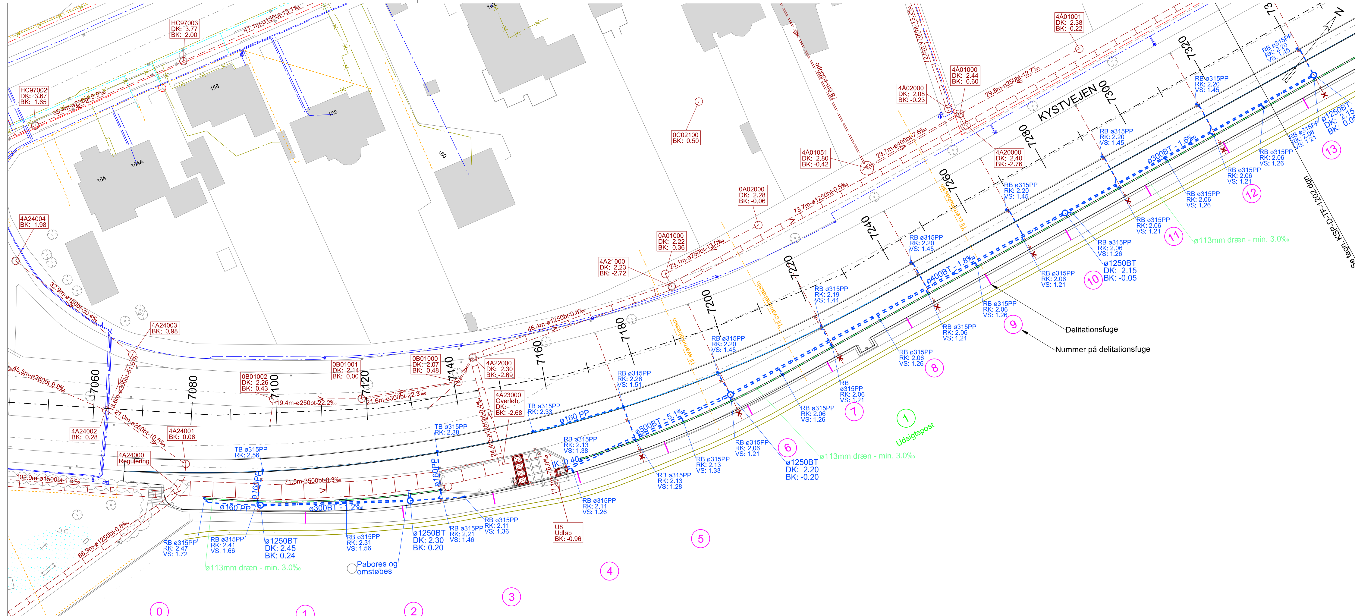
PLAN 1:500
